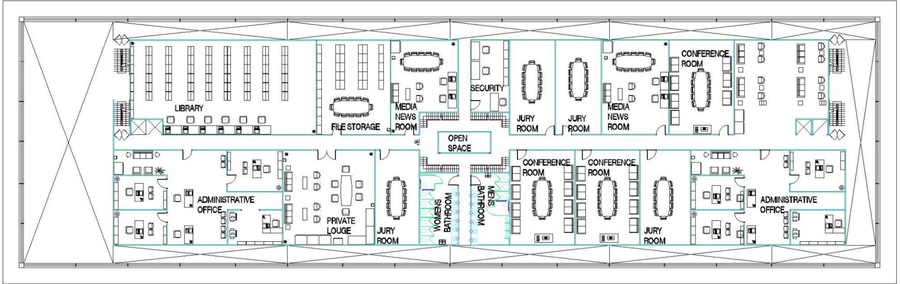
SECOND FLOOR
